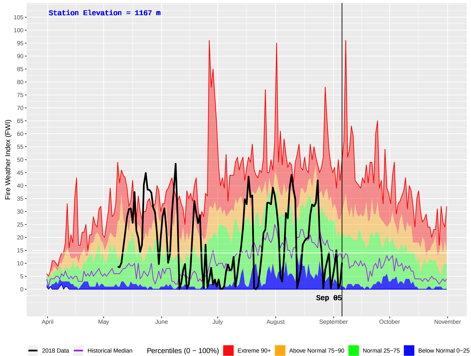
LEIGHTON LAKE (307) : Historical (1982–2016) and Current (2018) Daily Fire Weather Index (FWI)
