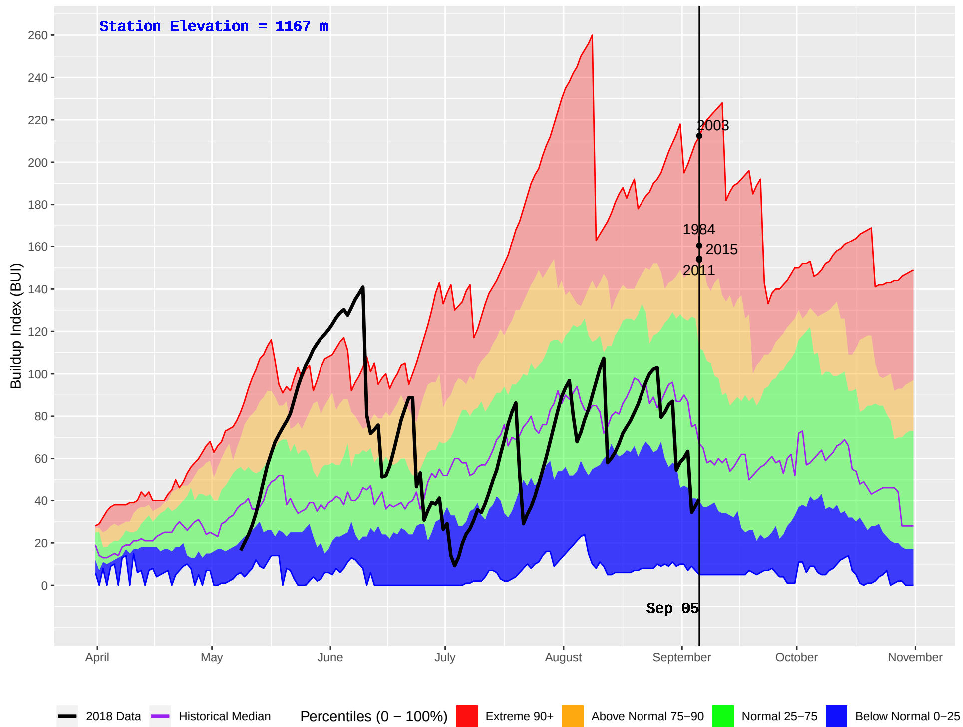
LEIGHTON LAKE (307) : Historical (1982–2016) and Current (2018) Daily Buildup Index (BUI)
