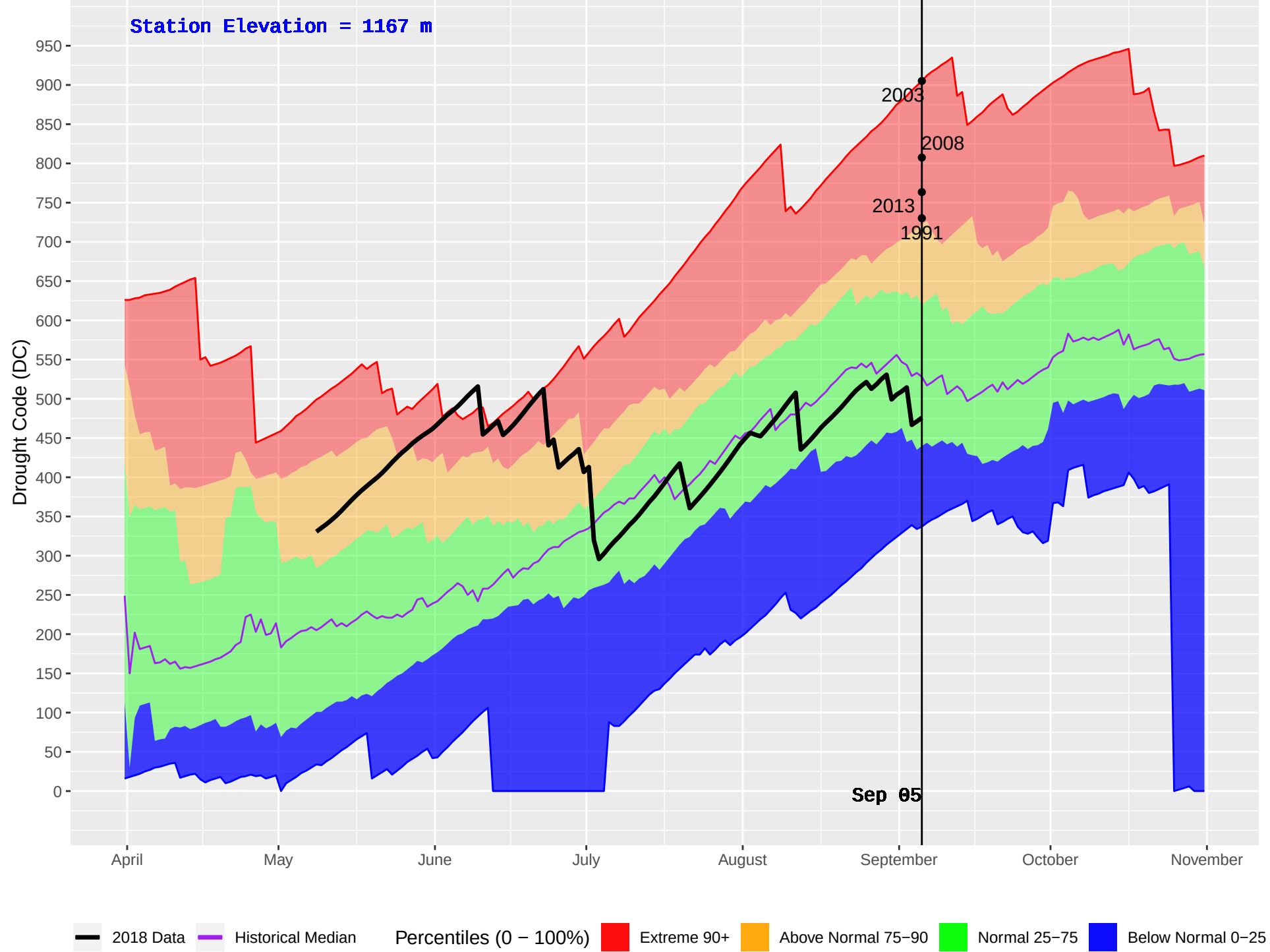
LEIGHTON LAKE (307) : Historical (1982–2016) and Current (2018) Daily Drought Code (DC)
