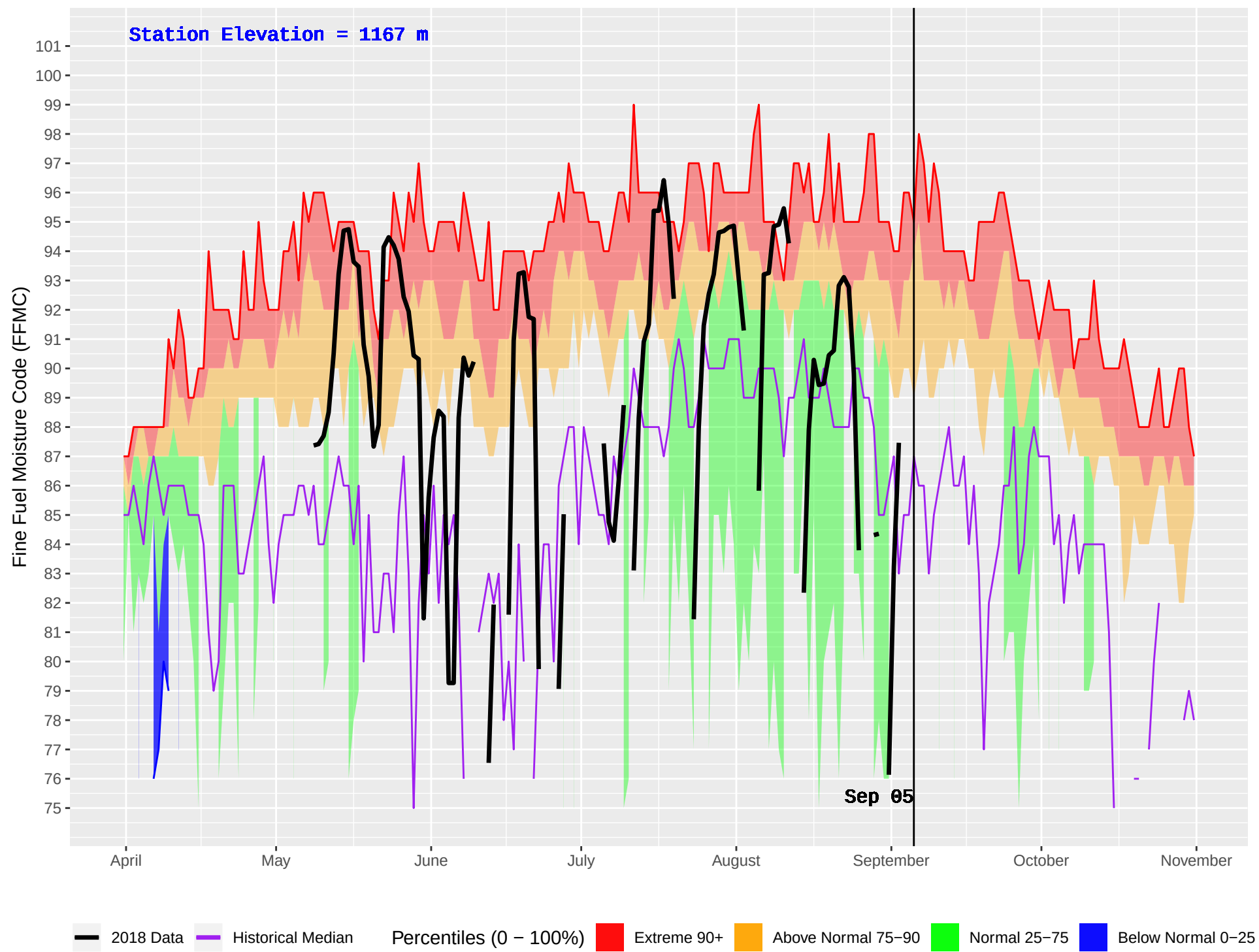
LEIGHTON LAKE (307) : Historical (1982–2016) and Current (2018) Daily Fine Fuel Moisture Code (FFMC)
