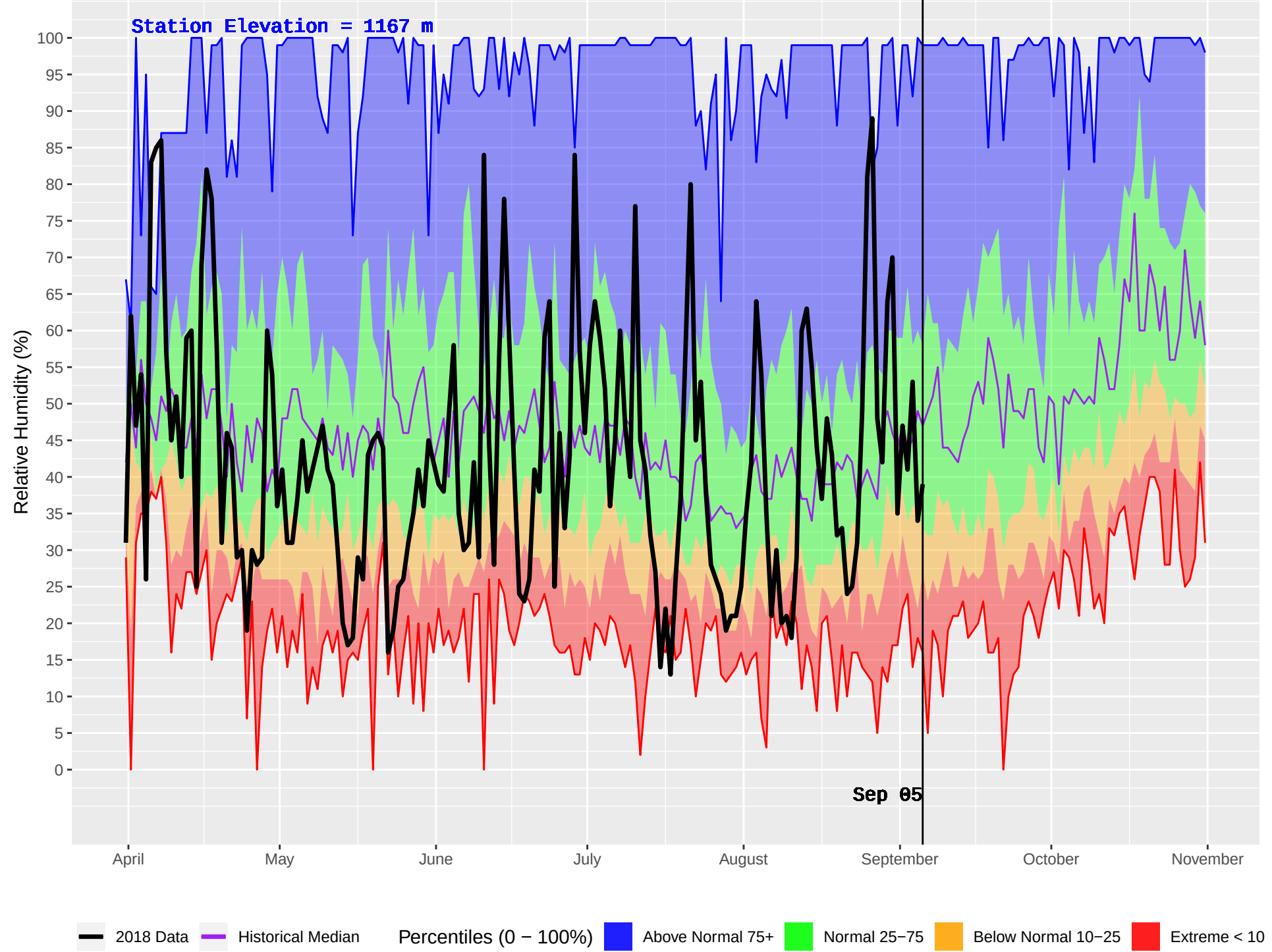
LEIGHTON LAKE (307) : Historical (1982–2016) and Current (2018) Daily Relative Humidity
