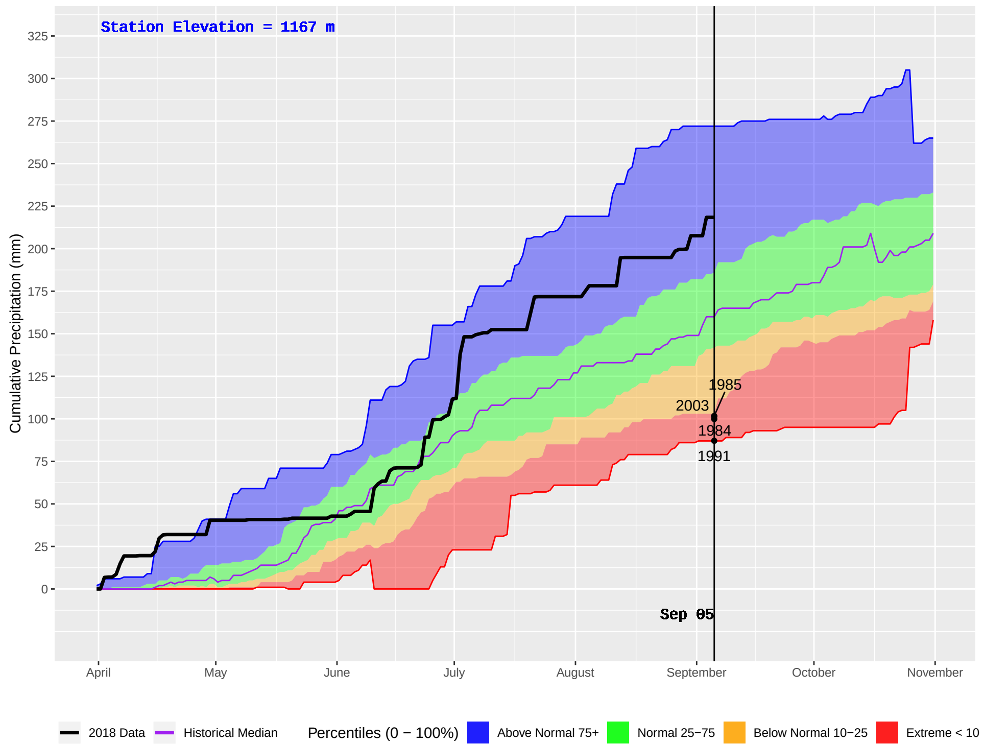
LEIGHTON LAKE (307) : Historical (1982–2016) and Current (2018) Daily Cumulative Precipitation
