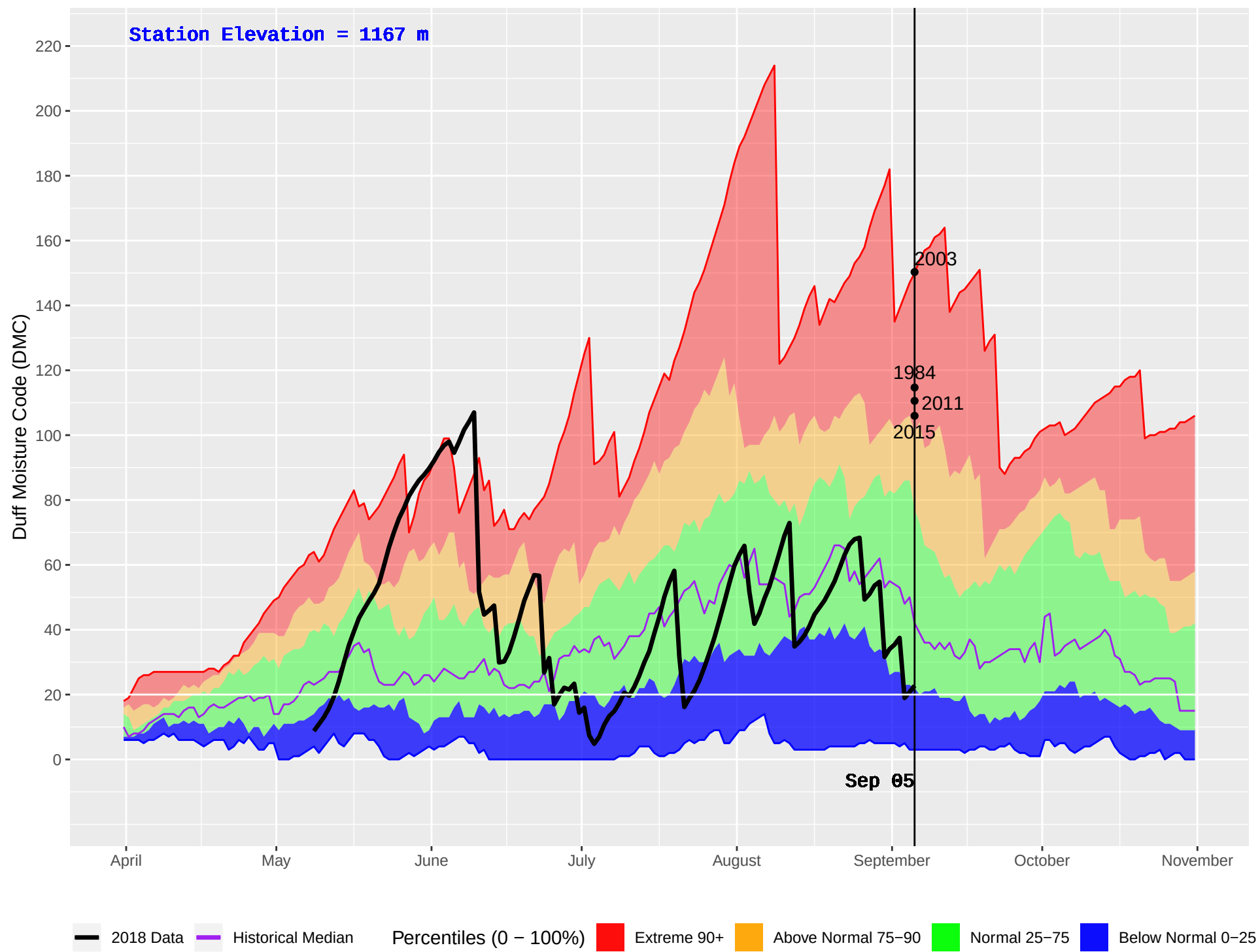
LEIGHTON LAKE (307) : Historical (1982–2016) and Current (2018) Daily Duff Moisture Code (DMC)
