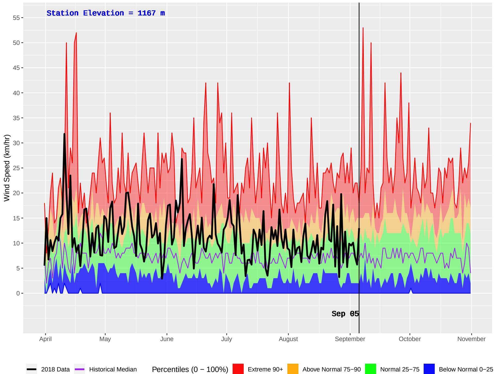
LEIGHTON LAKE (307) : Historical (1982–2016) and Current (2018) Daily Wind Speed
